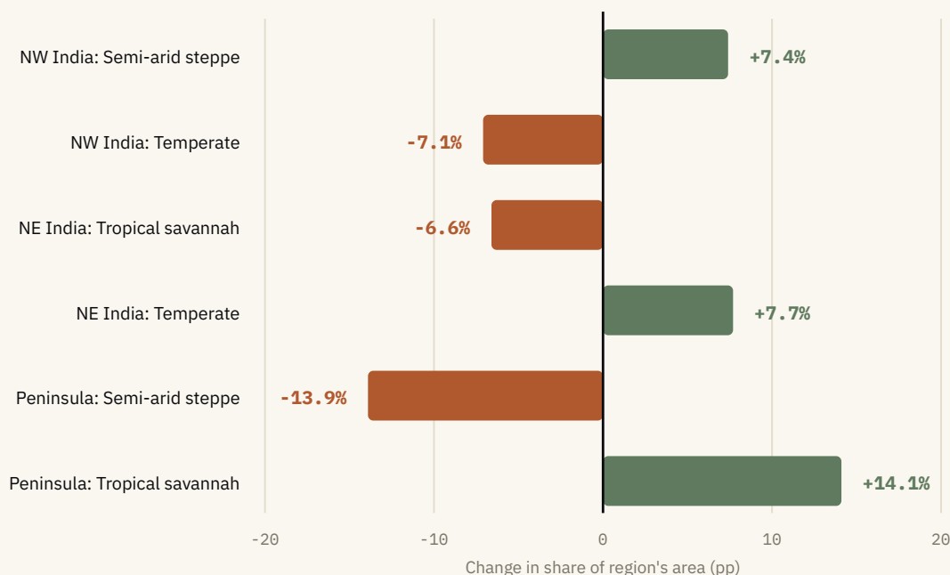
Climate-Zone Area Change, 1951-80 to 1991-2020 (percentage points)
